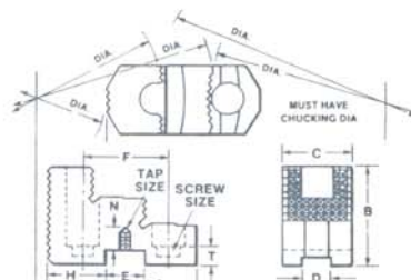
ACME SERRATED HARD JAW
