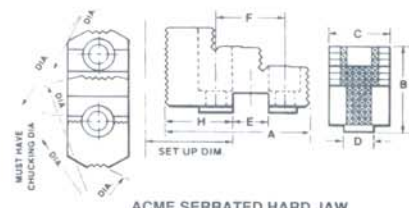
ACME SERRATED HARD JAW
