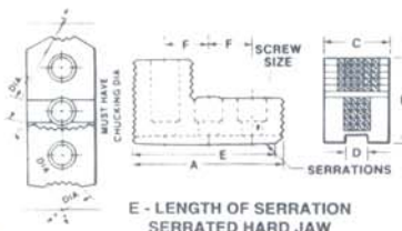
*SERRATIONS 3mm x 60° E - LENGTH OF SERRATION (.1181)
