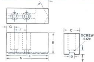
*SERRATIONS 1.5mm x 60° E - LENGTH OF SERRATION (.0591)
