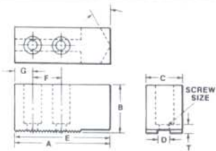
*SERRATIONS 3mm x 60° E - LENGTH OF SERRATION (.1181)
