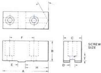
AMERICAN STANDARD TONGUE & GROOVE
