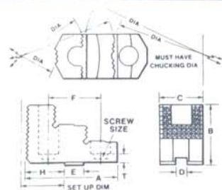
E - LENGTH OF SERRATION SERRATED HARD JAW
