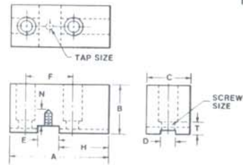
SQUARE SERRATED
