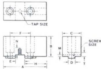
ACME SERRATED
